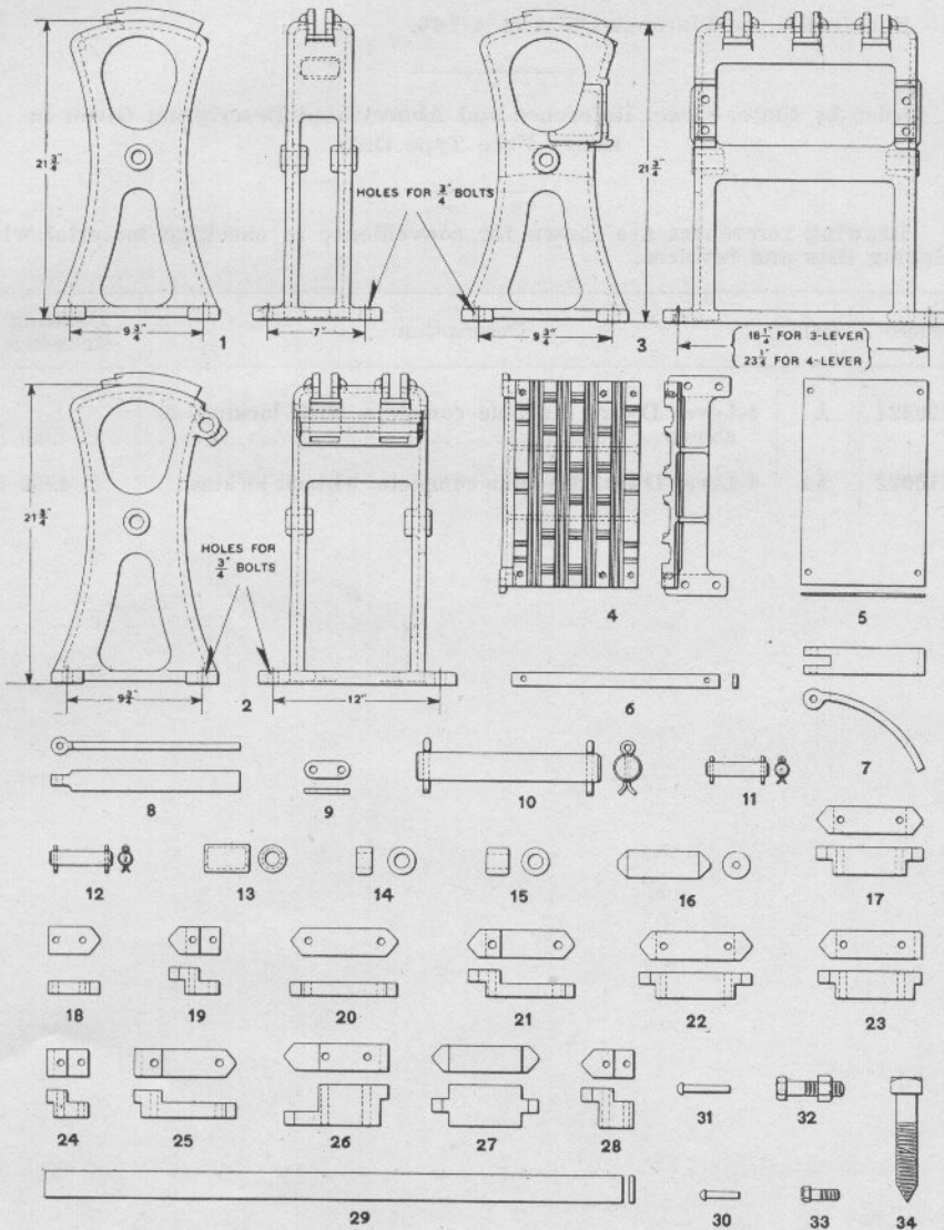
STANDS, LOCKING PLATES, TAPPETS, LOCKING DOGS, ETC., FOR DWARF INTERLOCKING MACHINE
